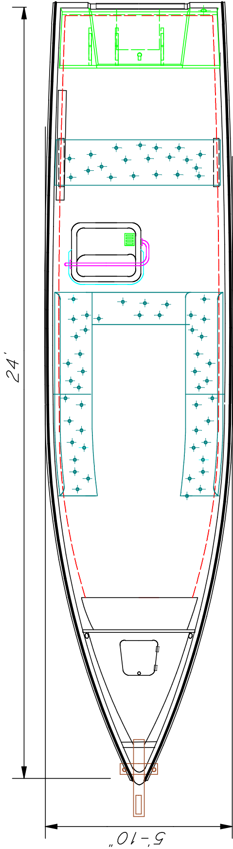
MAIN DECK PLAN
