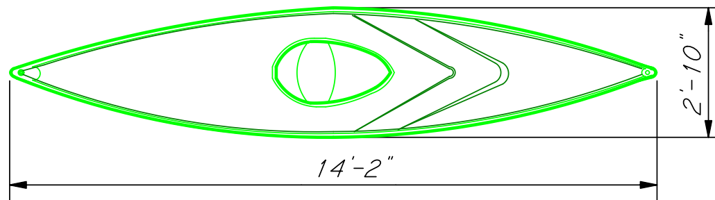
PLAN VIEW
