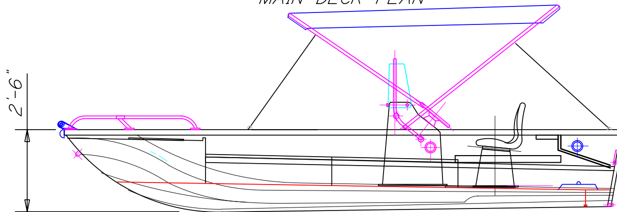
INBOARD PROFILE
