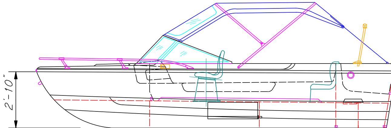
INBOARD PROFILE
