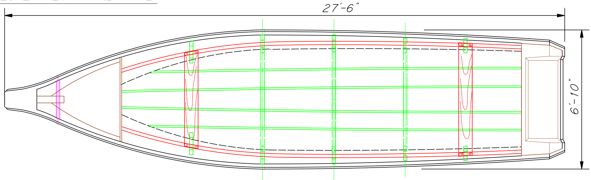
MAIN DECK PLAN
