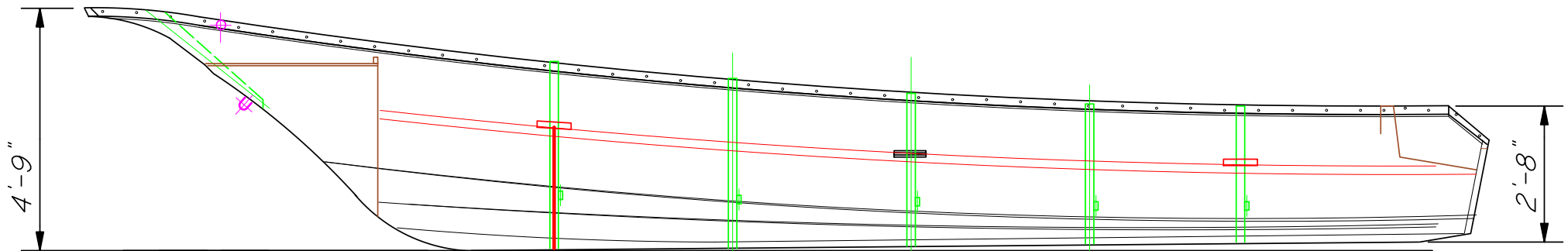
INBOARD PROFILE
