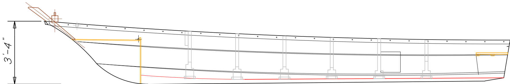
INBOARD PROFILE
