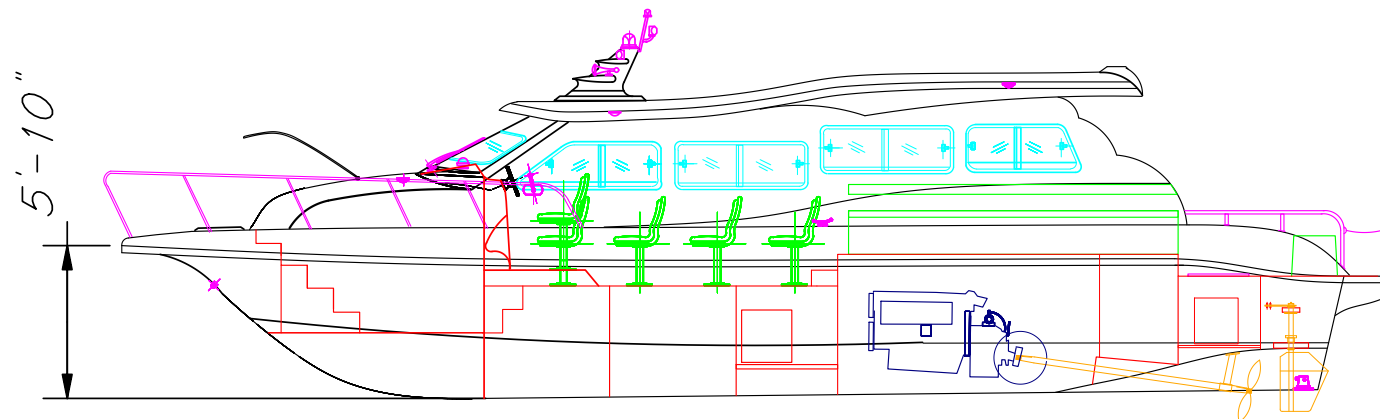
INBOARD PROFILE
