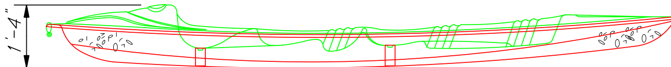
INBOARD PROFILE
