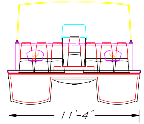
BODY PLAN
