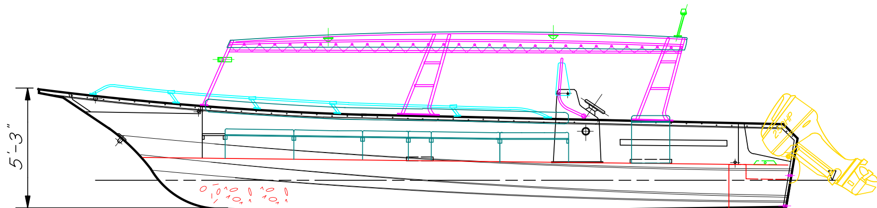
INBOARD PROFILE
