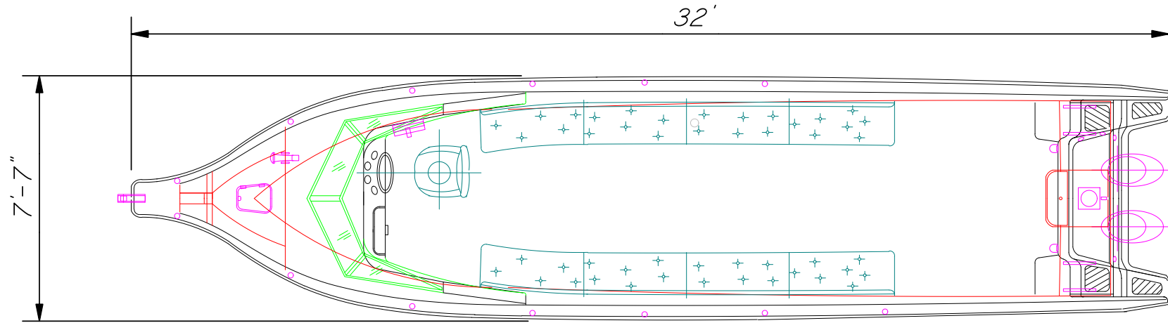
MAIN DECK PLAN
