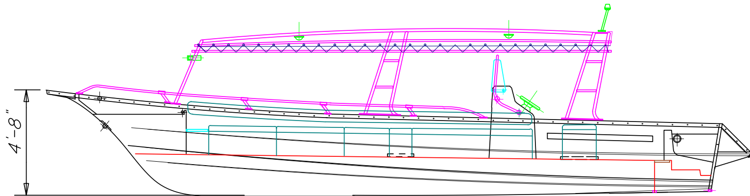
INBOARD PROFILE
