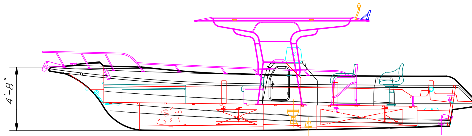
INBOARD PROFILE
