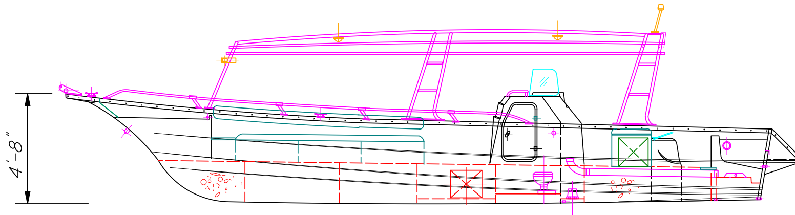
INBOARD PROFILE
