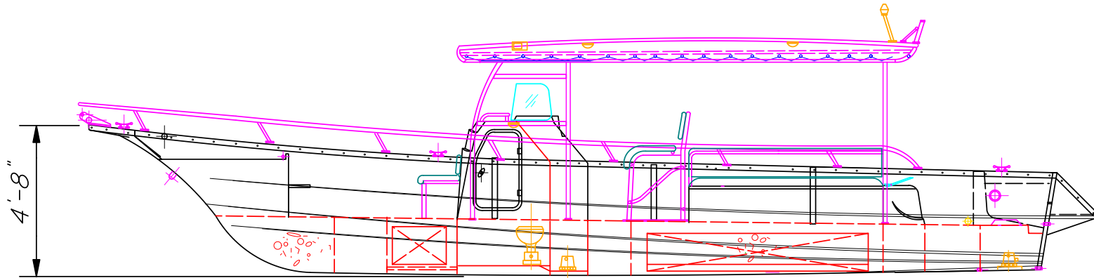
INBOARD PROFILE
