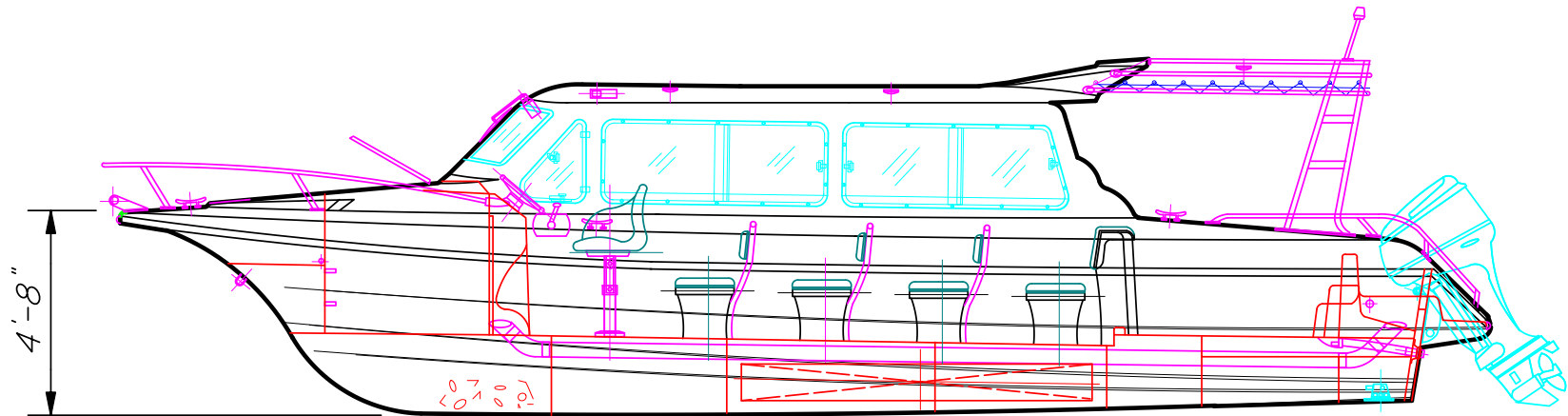
INBOARD PROFILE
