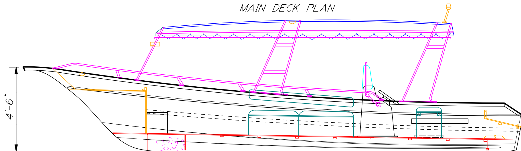
INBOARD PROFILE
