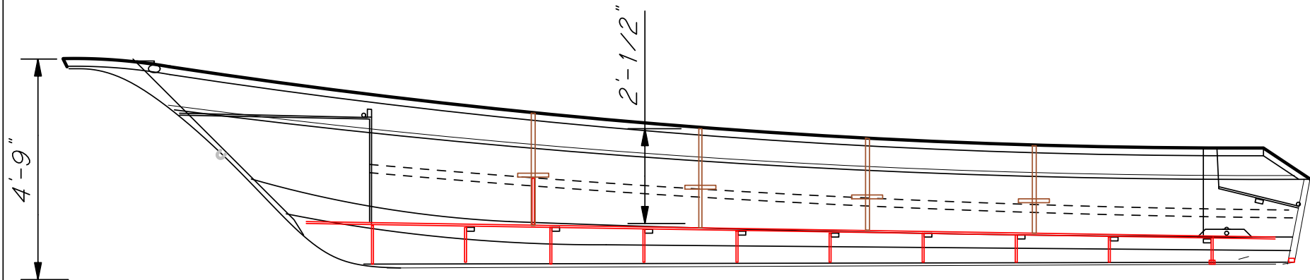
INBOARD PROFILE
