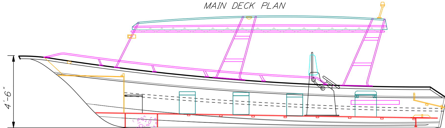
INBOARD PROFILE
