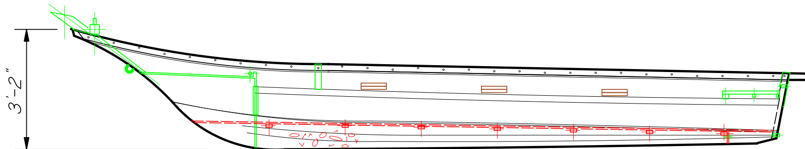
INBOARD PROFILE
