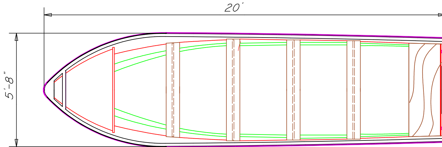
MAIN DECK PLAN
