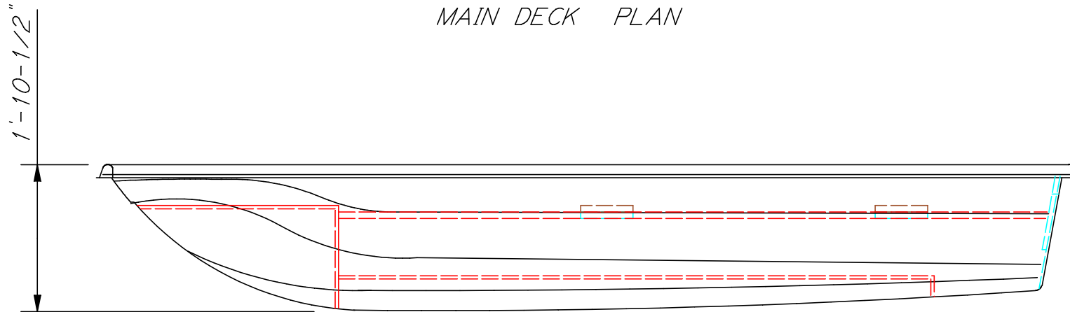
INBOARD PROFILE
