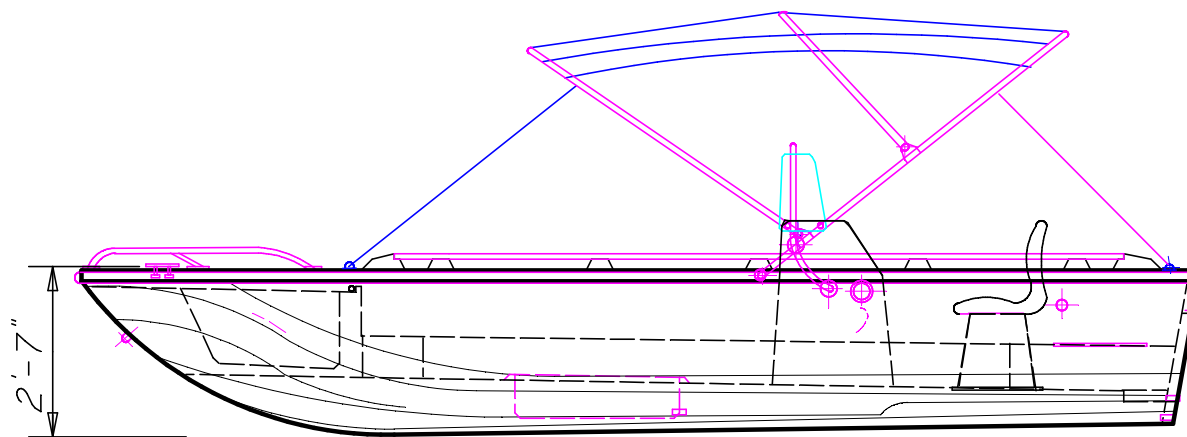
INBOARD PROFILE
