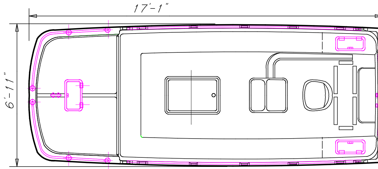
MAIN DECK PLAN
