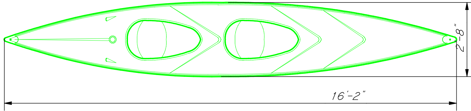
PLAN VIEW
