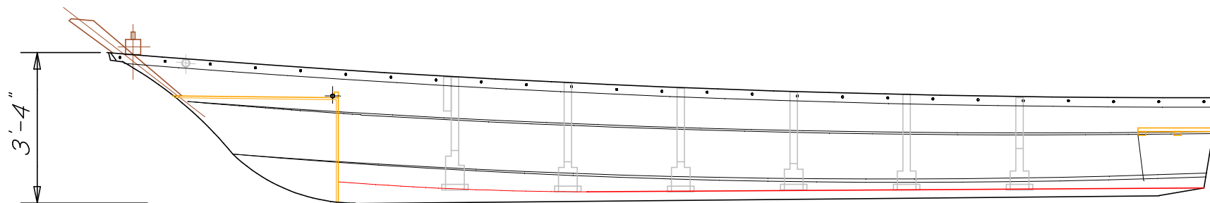
INBOARD PROFILE
