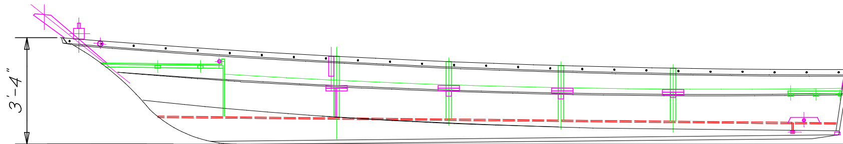
INBOARD PROFILE
