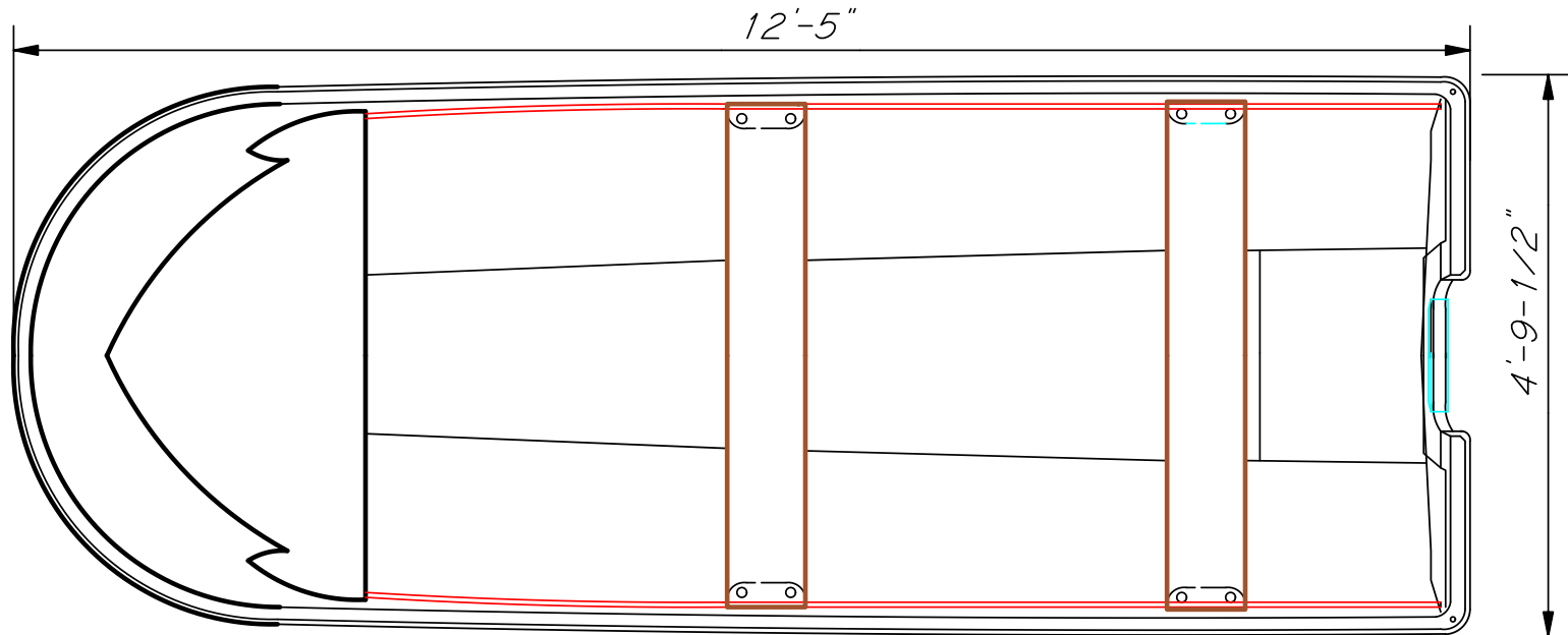
MAIN DECK PLAN
