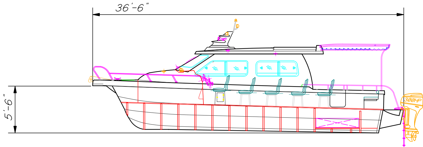
INBOARD PROFILE
