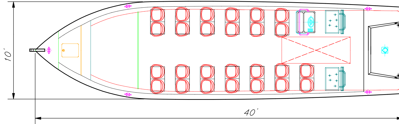
MAIN DECK PLAN
