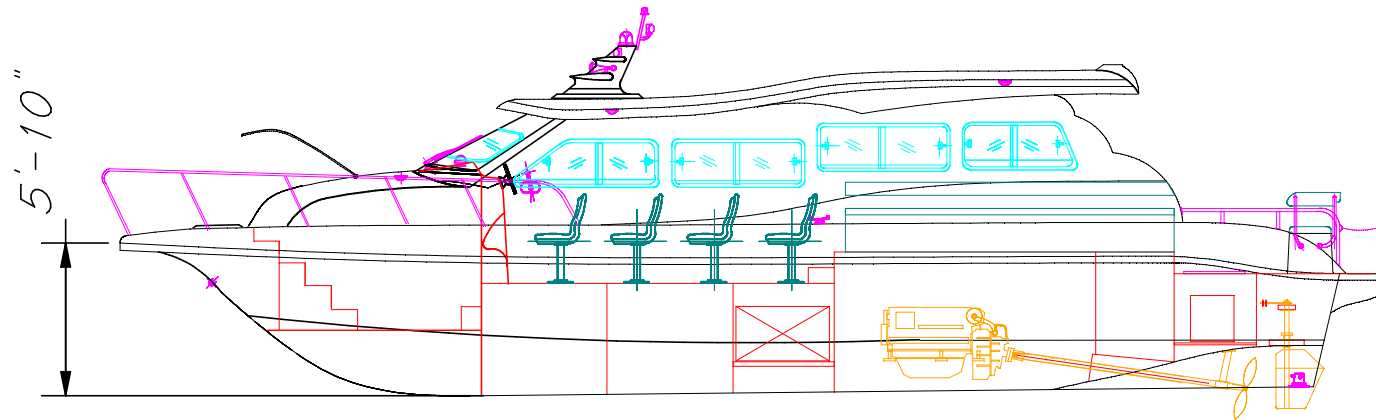
INBOARD PROFILE
