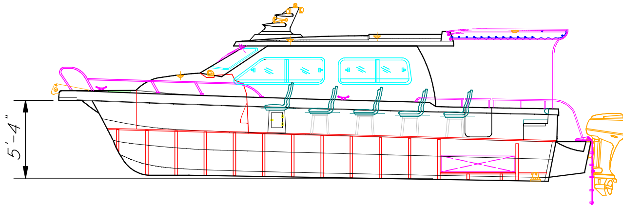
INBOARD PROFILE
