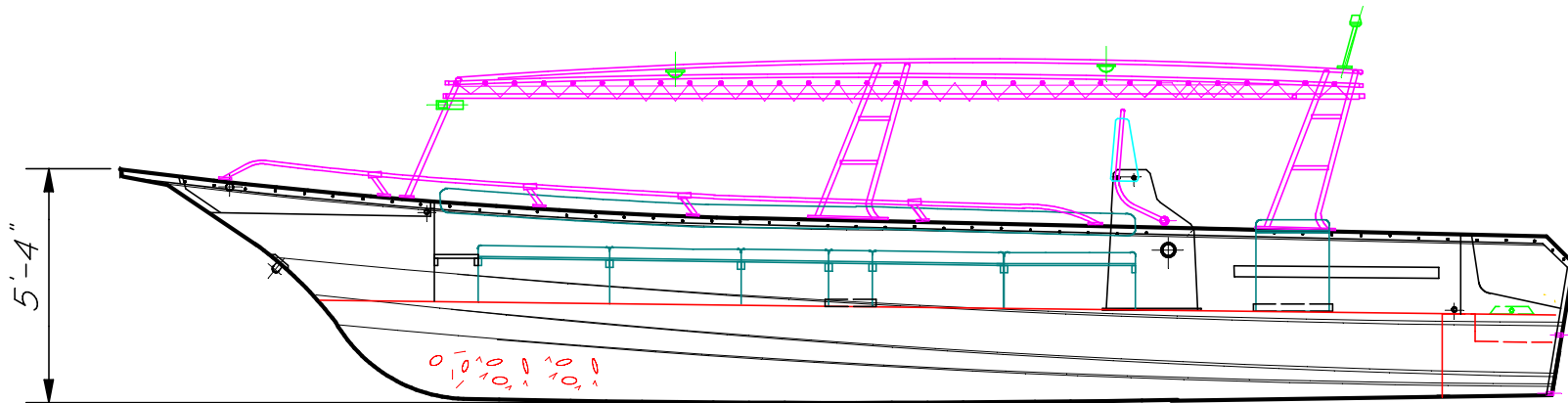
INBOARD PROFILE
