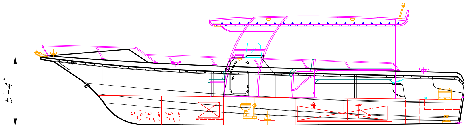
INBOARD PROFILE
