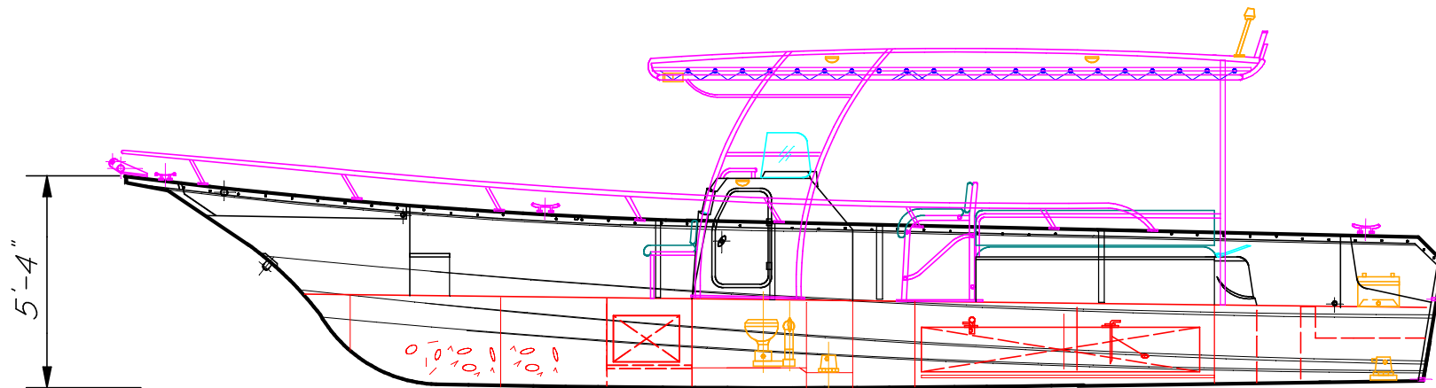
INBOARD PROFILE
