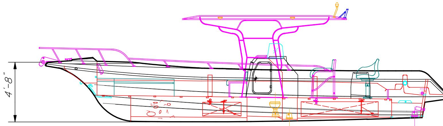
INBOARD PROFILE
