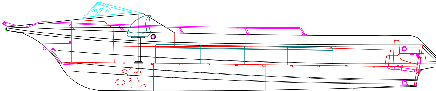
INBOARD PROFILE
