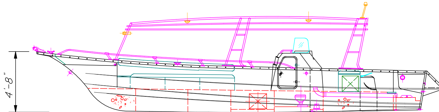
INBOARD PROFILE
