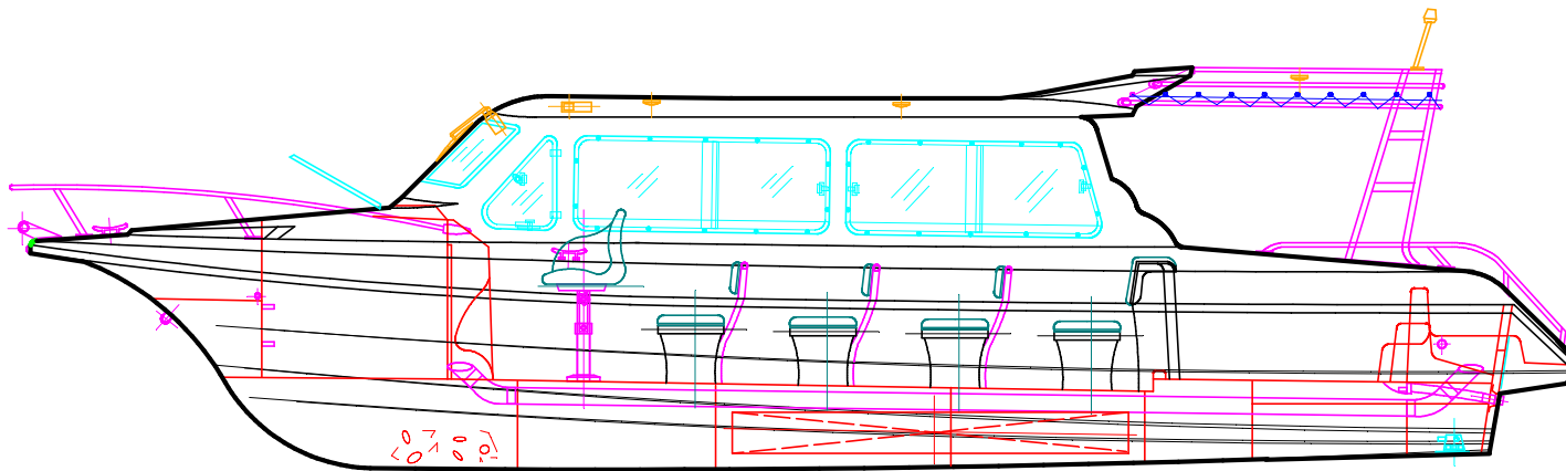
INBOARD PROFILE
