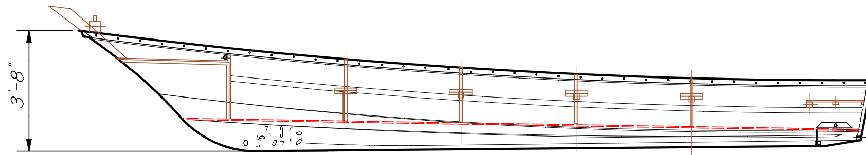
INBOARD PROFILE
