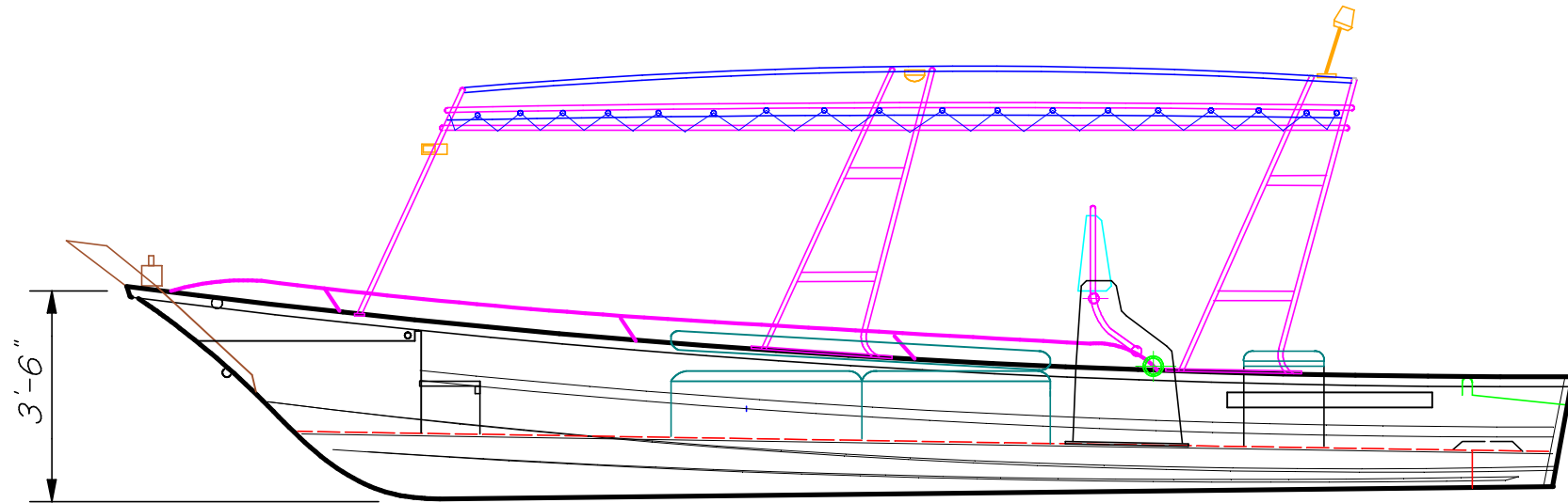
INBOARD PROFILE
